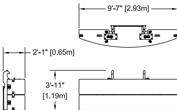
STANDARD COUNTERWEIGHT
